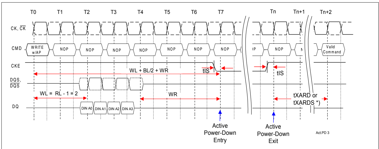
Figure 51 Active Power-Down Mode Entry and Exit Example after a Write Command with AP: WL = 2, WR = 3, BL = 4
