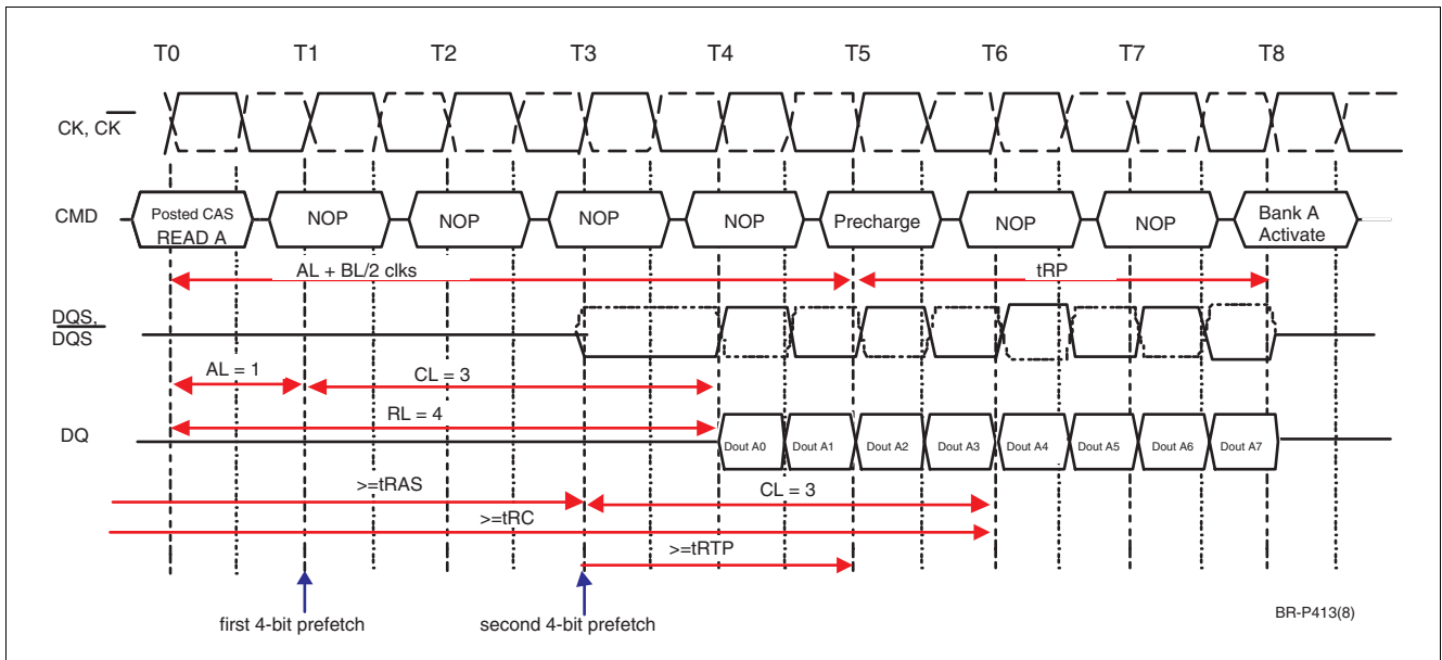
Figure 36 Read Operation Followed by Precharge Example 2: RL = 4 (AL = 1, CL = 3), BL = 8, t_{RTP} \leq 2 clocks
