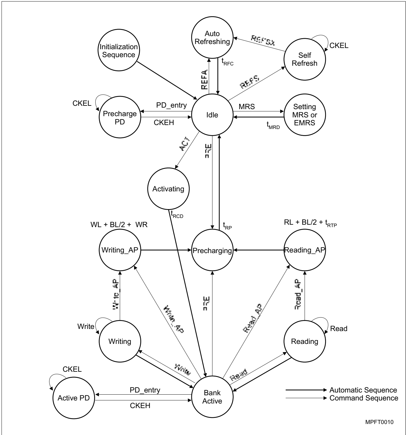
Figure 3 Simplified State Diagram
