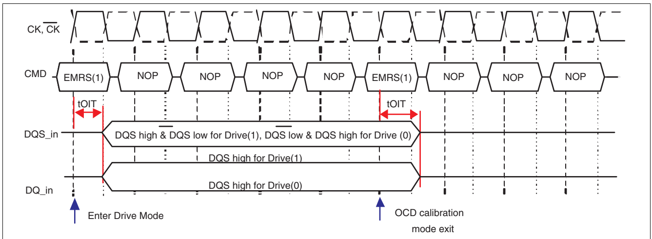
Figure 7 Timing Diagram Drive Mode
