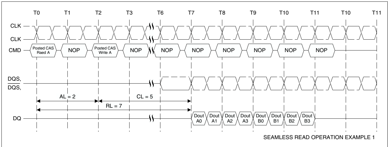
Figure 23 Seamless Read Operation Example 1: RL = 7, AL = 2, CL = 5, BL = 4
