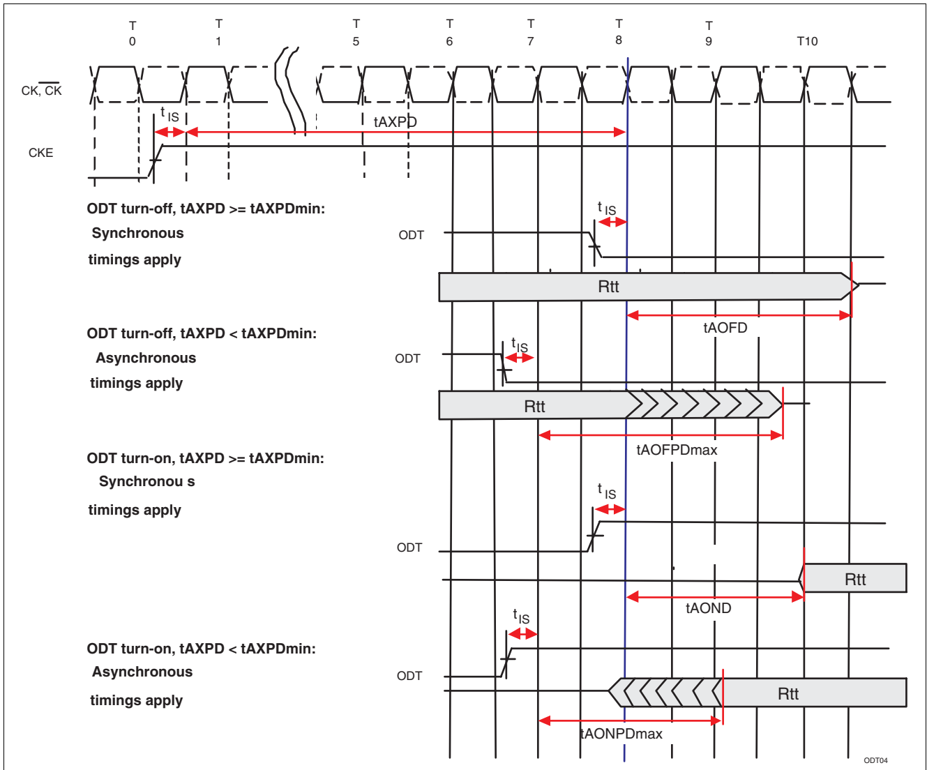
Figure 12 ODT Mode exit Timing Diagram
