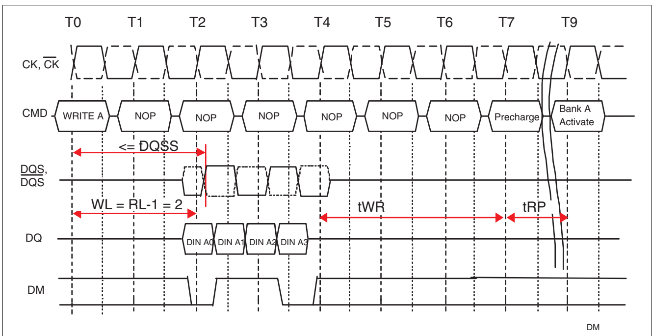
Figure 32 Write Operation with Data Mask Example: \text{RL} = 3 ( \text{AL} = 0, \text{CL} = 3 ), \text{WL} = 2, t_{\text{WR}} = 3, \text{BL} = 4
