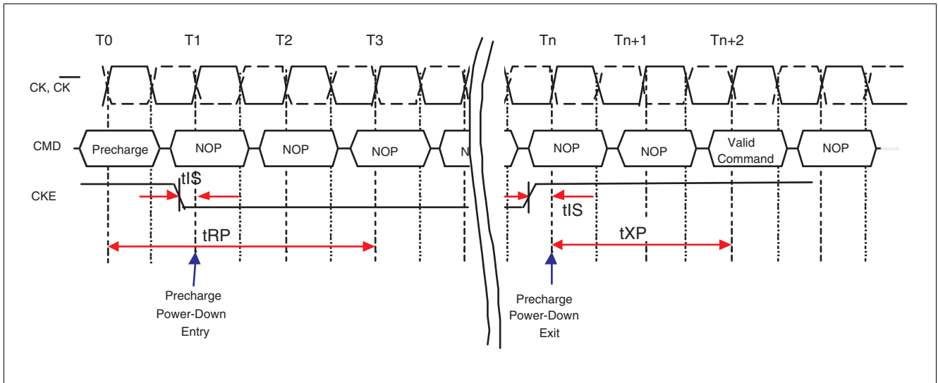
Figure 52 Precharge Power Down Mode Entry and Exit
