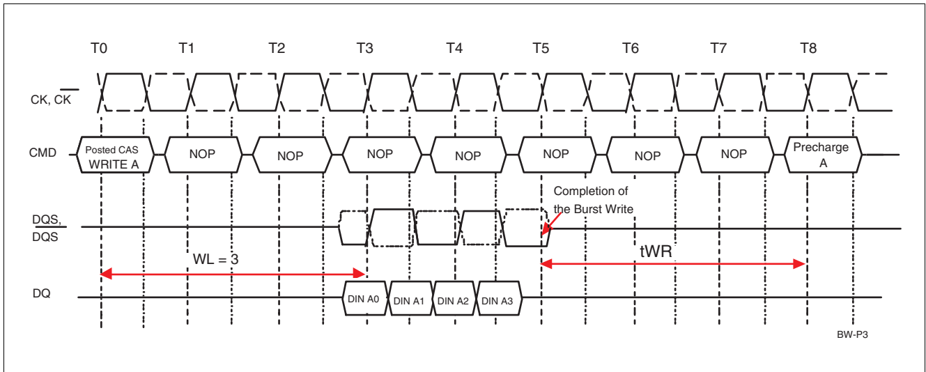
Figure 39 Write followed by Precharge Example 1: WL = (RL - 1) = 3 , BL = 4 , t_{WR} = 3
