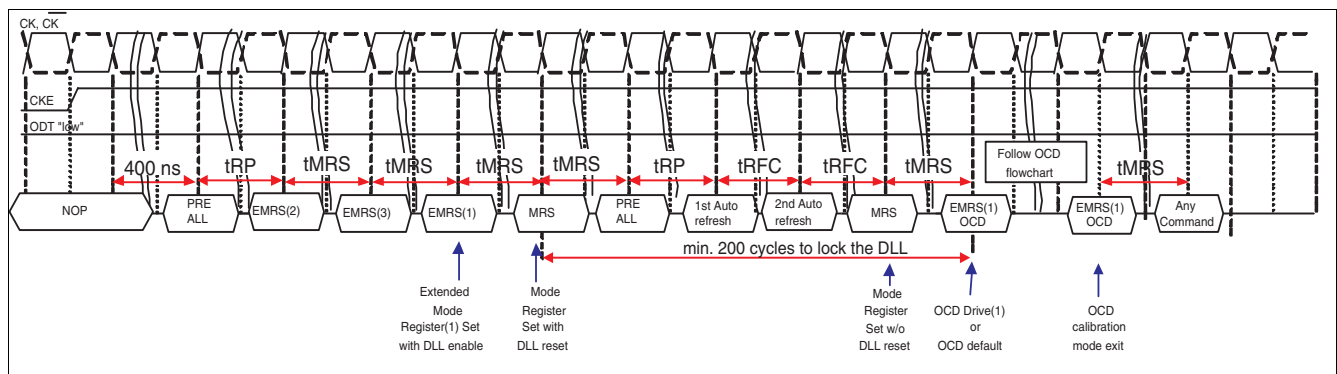
Figure 4 Initialization Sequence after Power Up
