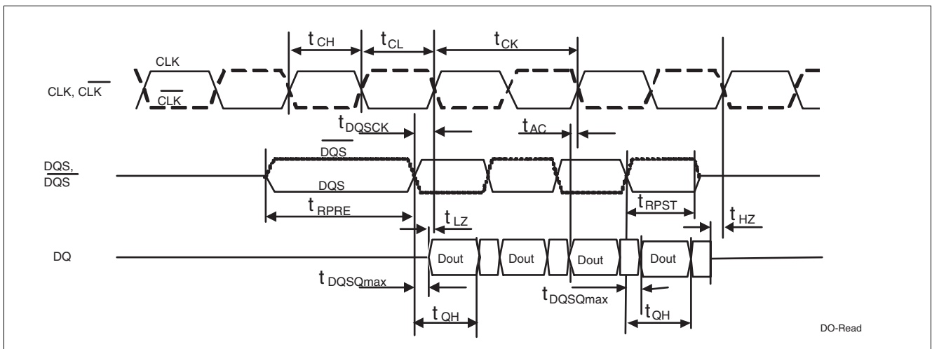
Figure 19 Basic Read Timing Diagram
