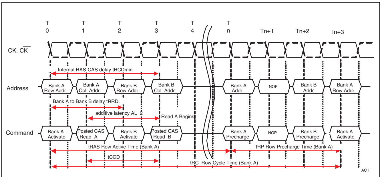
Figure 13 Bank Activate Command Cycle: t_{\text{RCD}} = 3 , AL = 2 , t_{\text{RP}} = 3 , t_{\text{RRD}} = 2
