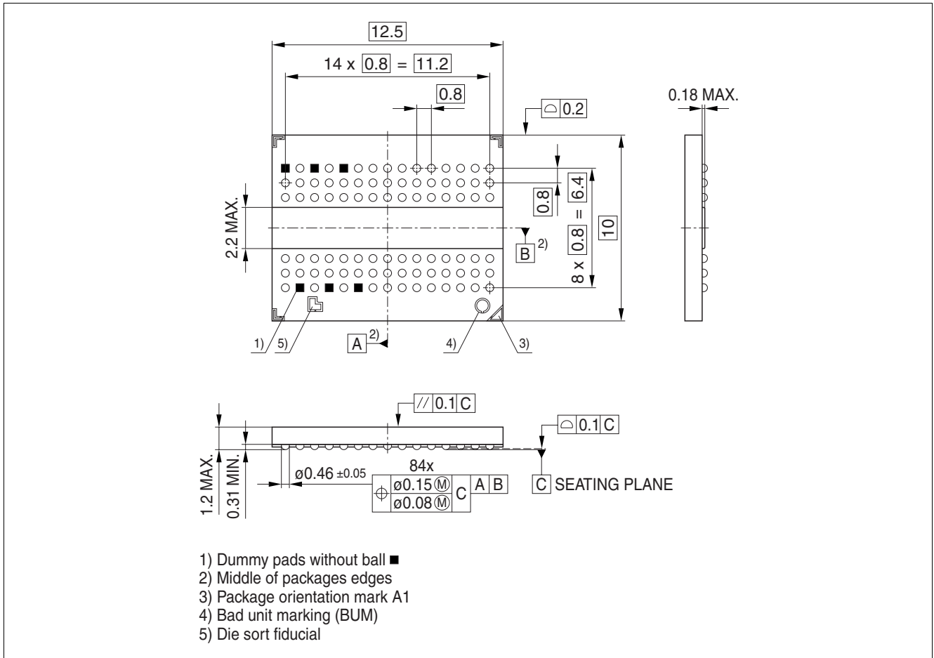
Figure 69 Package Pinout PG-TFBGA-84-3 (top view)
