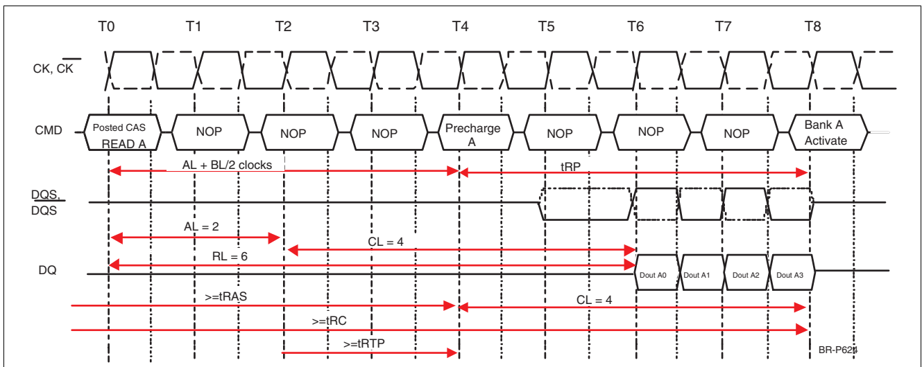
Figure 38 Read Operation Followed by Precharge Example 4: RL = 6, (AL = 2, CL = 4), BL = 4, t_{RTP} \leq 2 clocks
