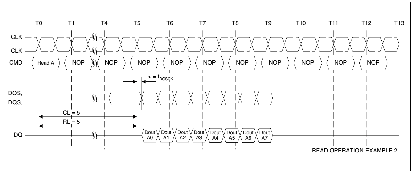
Figure 21 Read Operation Example 2: RL = 5 ( AL = 0 , CL = 5 , BL = 8 )
