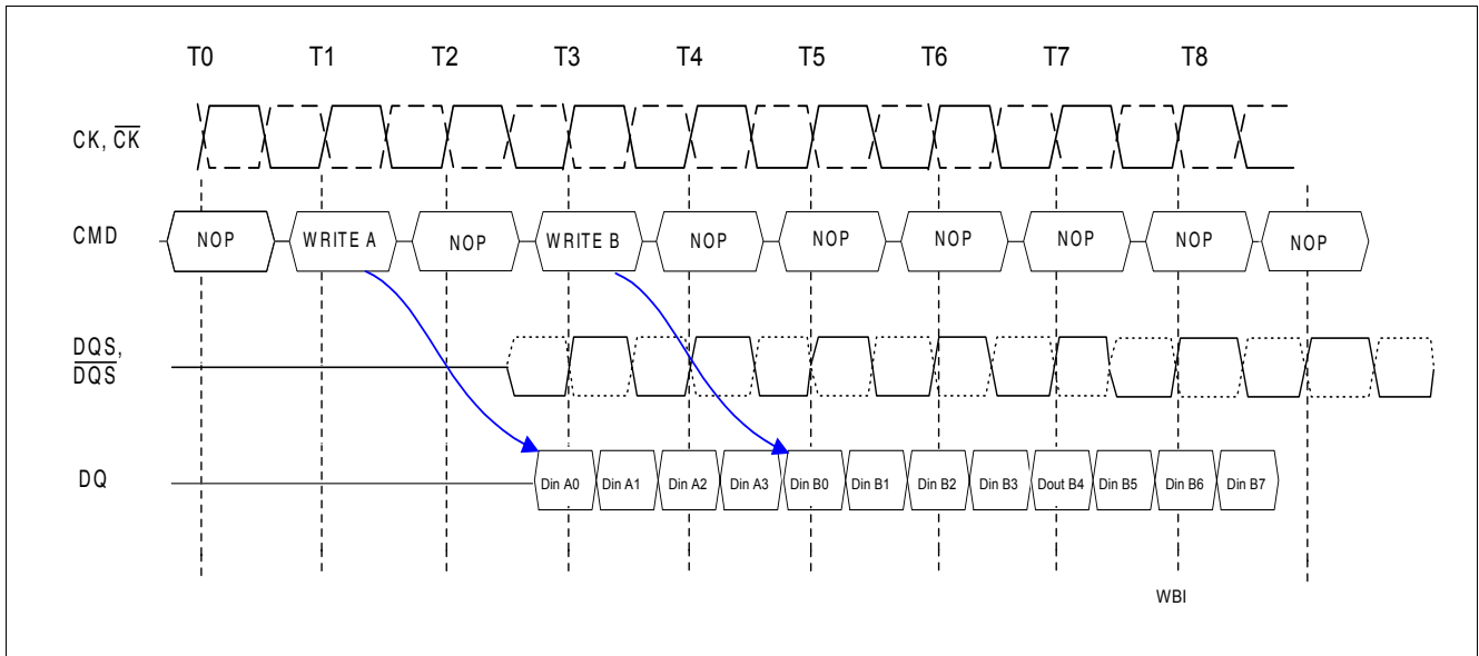
Figure 34 Write Interrupt Timing Example 2: (CL = 3, AL = 0, WL = 2, BL = 8)
