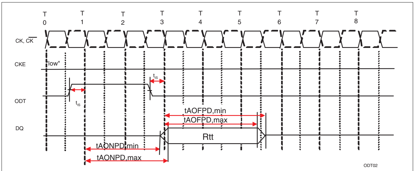
Figure 10 ODT Timing for Precharge Power-Down and Active Power-Down Mode (with slow exit) (Asynchronous ODT timings)
