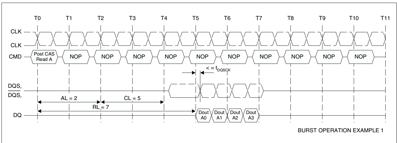
Figure 20 Read Operation Example 1: RL = 7 (AL = 2, CL = 5, BL = 4)
