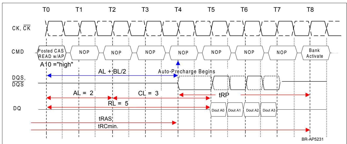
Figure 41 Read with Auto-Precharge Example 1, followed by an Activation to the Same Bank ( t_{\text{RC}} Limit): RL = 5 (AL = 2, CL = 3), BL = 4, t_{\text{RTP}} \leq 2 clocks
