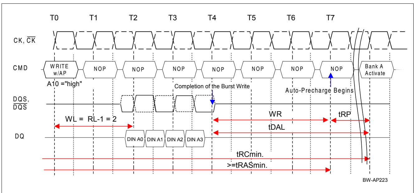
Figure 44 Write with Auto-Precharge Example 1 ( t_{RC} Limit): WL = 2 , t_{DAL} = 6 ( WR = 3 , t_{RP} = 3 ), BL = 4
