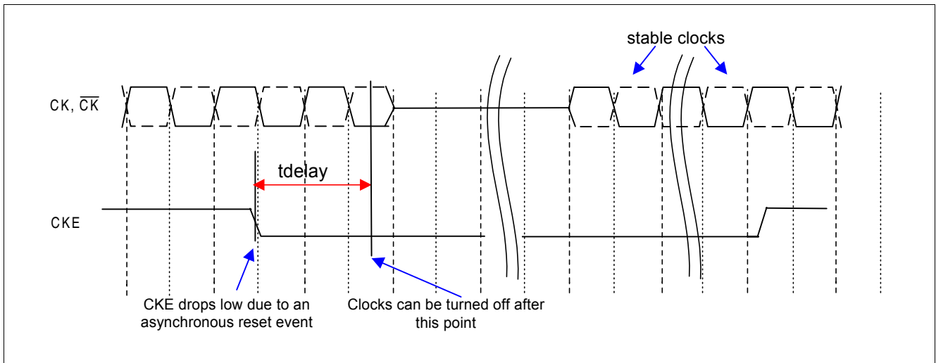
Figure 56 Asynchronous Low Reset Event
