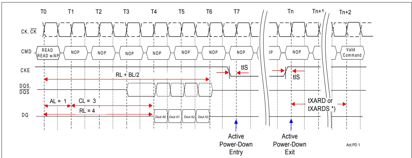
Figure 49 Active Power-Down Mode Entry and Exit Example after a Read Command: RL = 4 (AL = 1, CL = 3), BL = 4
