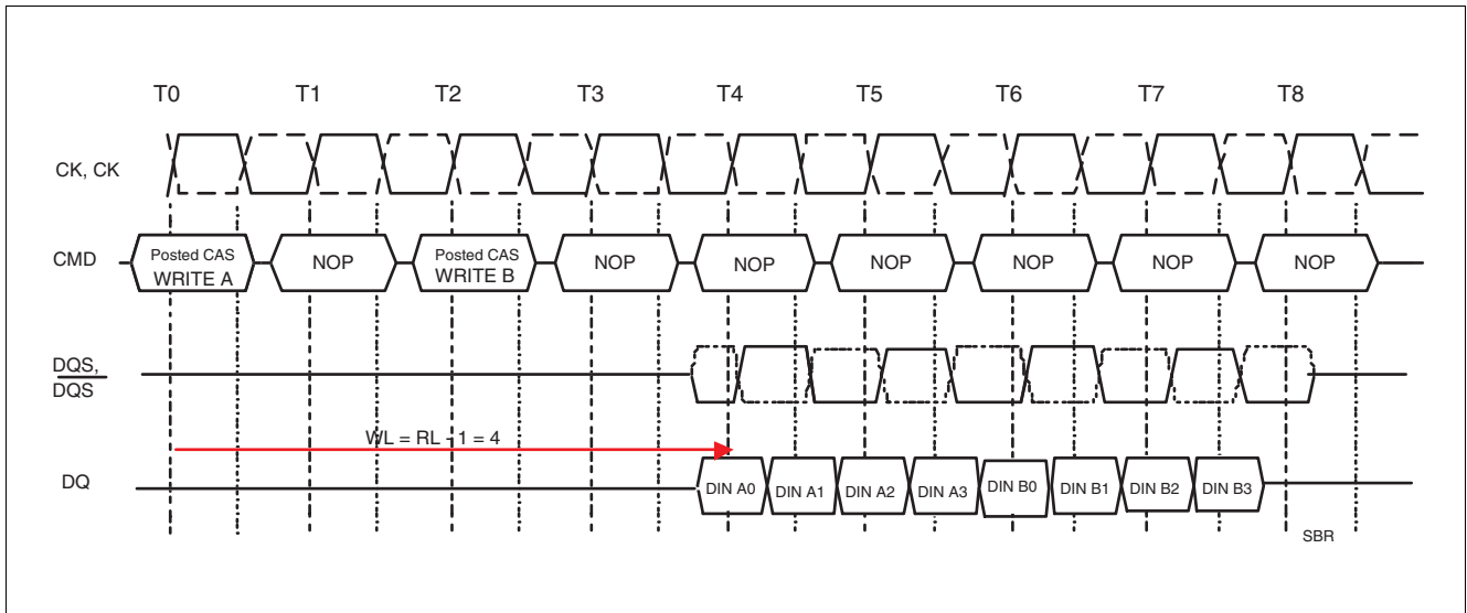
Figure 29 Seamless Write Operation Example 1: RL = 5 , WL = 4 , BL = 4
