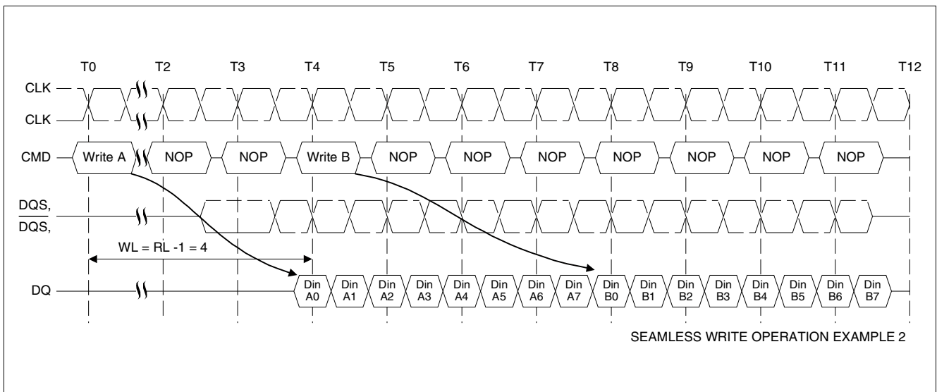
Figure 30 Seamless Write Operation Example 2: RL = 3 , WL = 4 , BL = 8 , non interrupting
