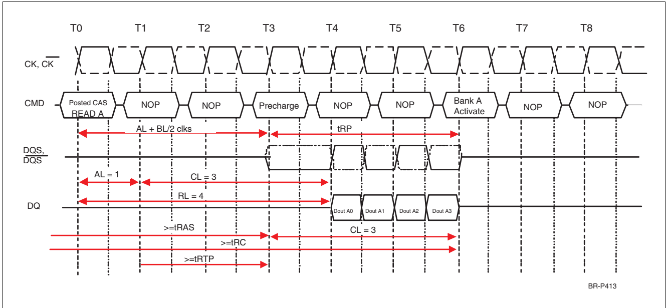
Figure 35 Read Operation Followed by Precharge Example 1: RL = 4 (AL = 1, CL = 3), BL = 4, t_{RTP} \leq 2 clocks
