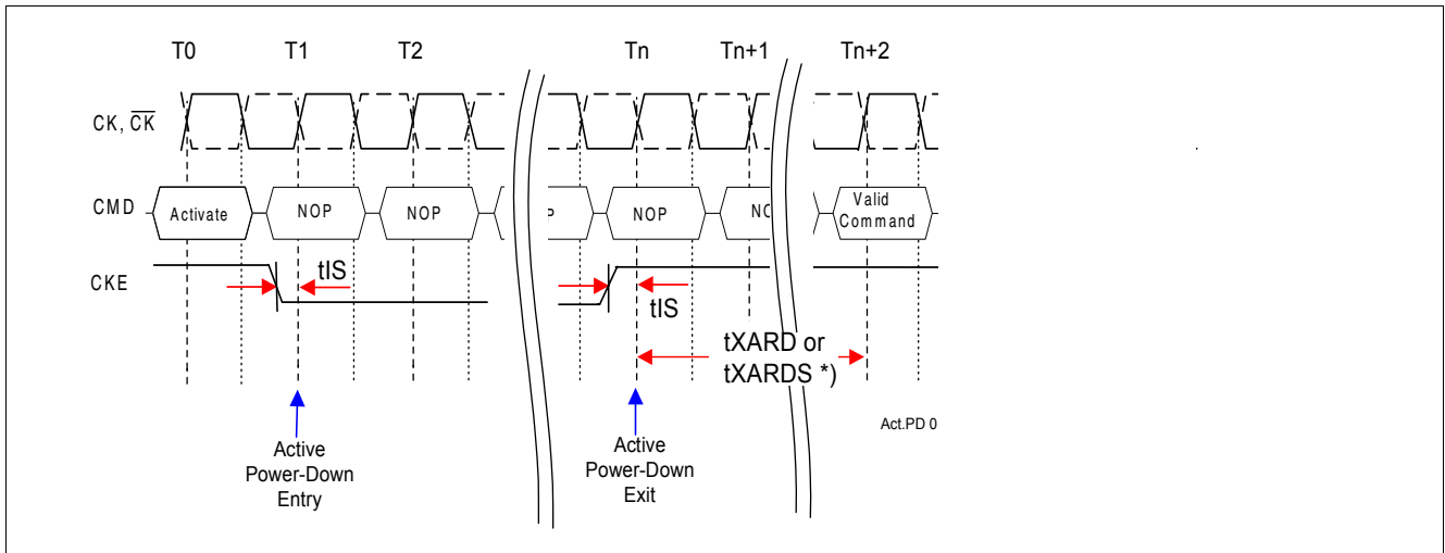
Figure 48 Active Power-Down Mode Entry and Exit after an Activate Command
