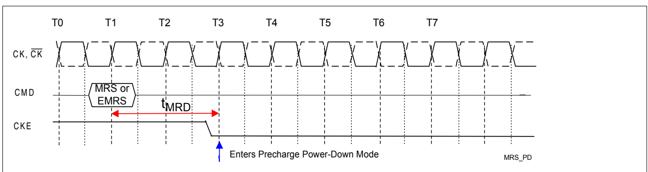
Figure 54 MRS, EMRS command to Power-Down entry
