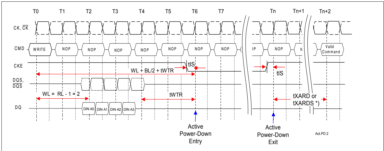
Figure 50 Active Power-Down Mode Entry and Exit Example after a Write Command: WL = 2, t_{WTR} = 2 , BL = 4
