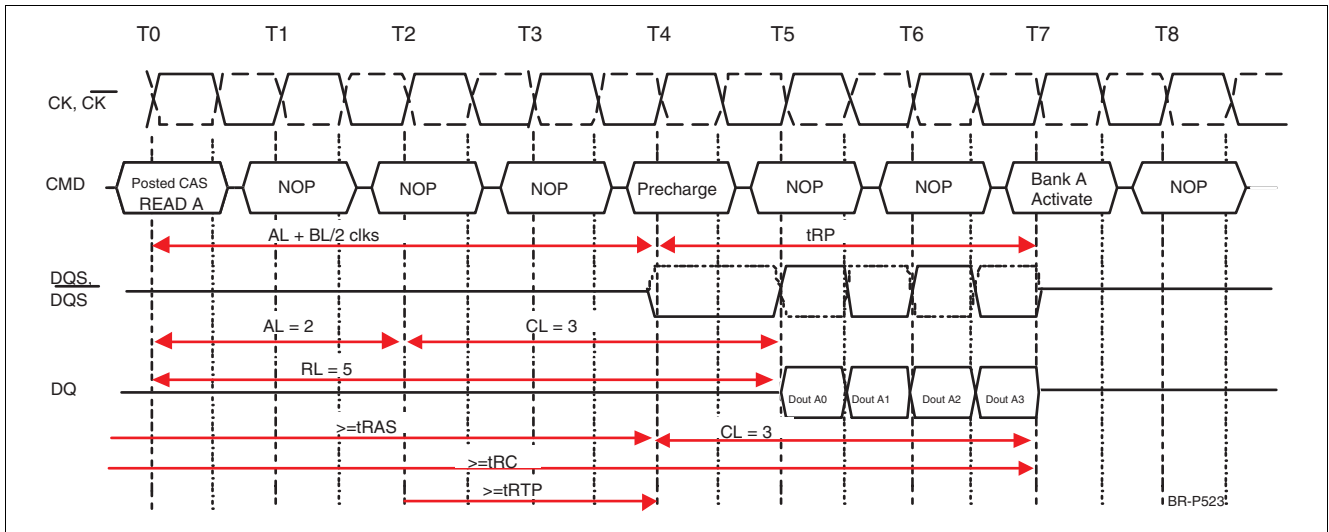
Figure 37 Read Operation Followed by Precharge Example 3: RL = 5 (AL = 2, CL = 3), BL = 4, t_{RTP} \leq 2 clocks
