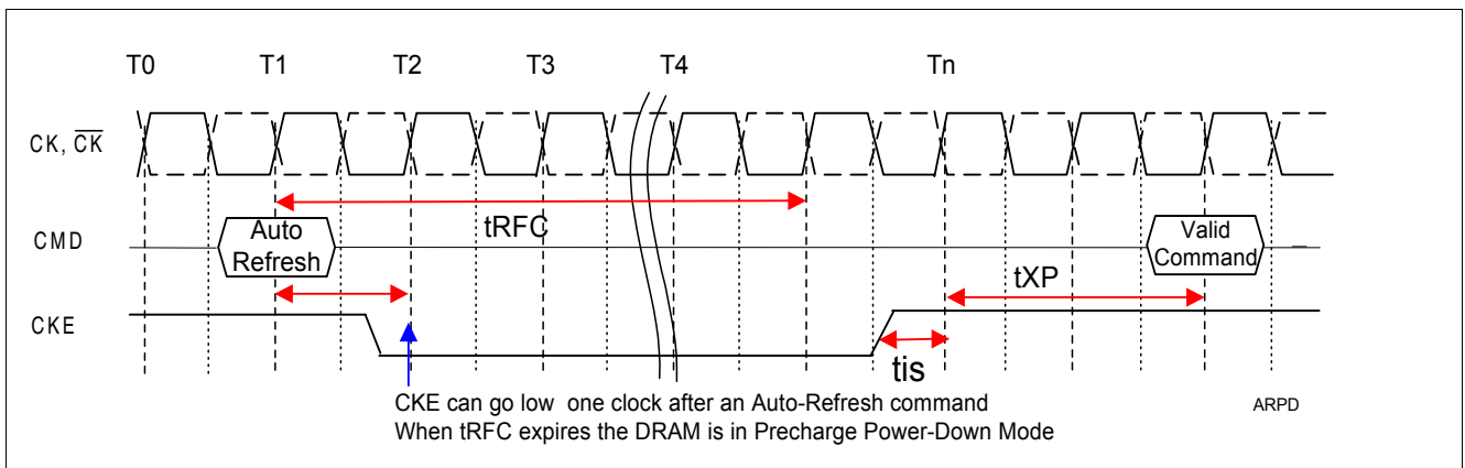
Figure 53 Auto-Refresh command to Power-Down entry
