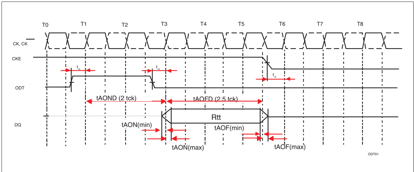
Figure 9 ODT Timing for Active and Standby (Idle) Modes (Synchronous ODT timings)
