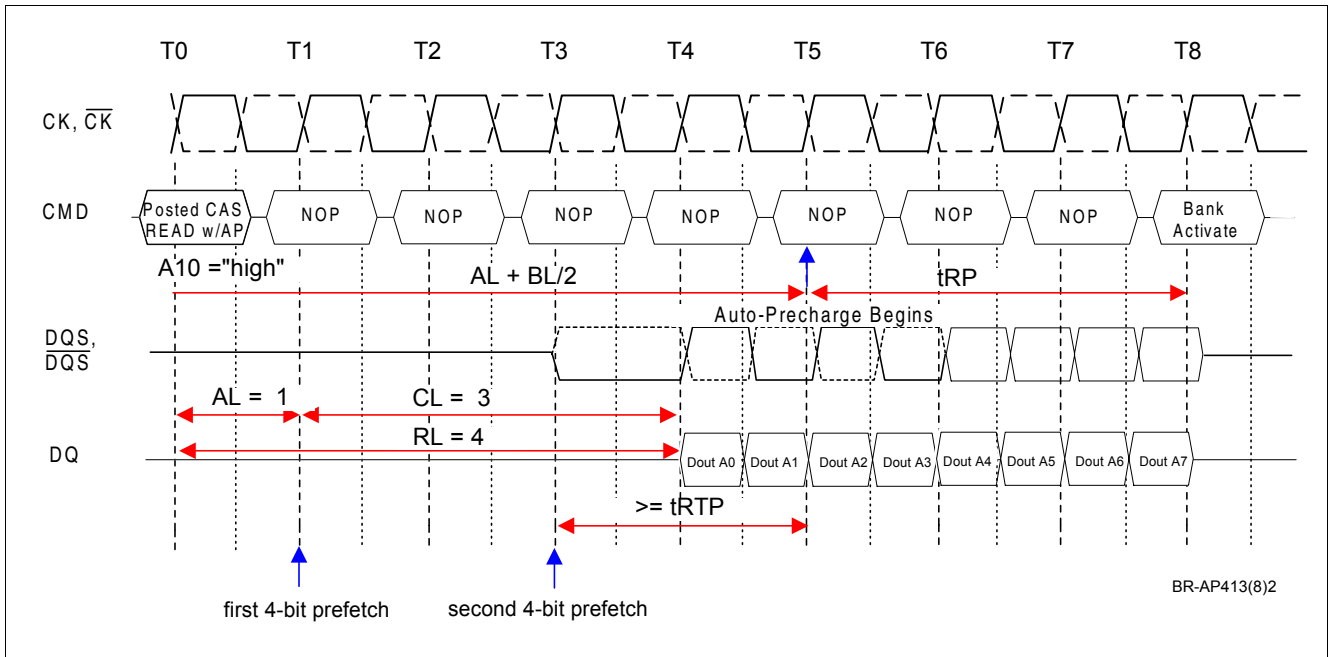
Figure 43 Read with Auto-Precharge Example 3, followed by an Activation to the Same Bank: RL = 4 (AL = 1, CL = 3), BL = 8, t_{RTP} \leq 2 clocks
