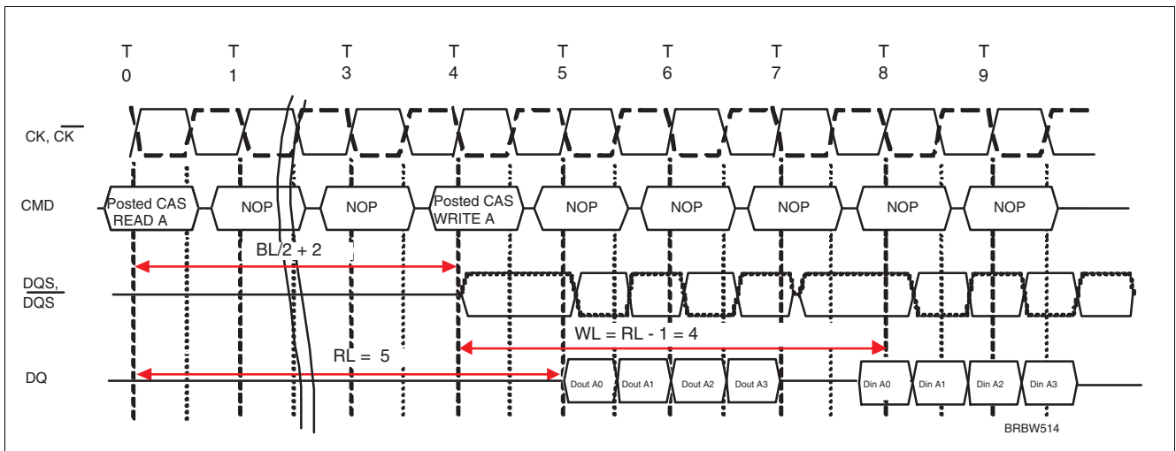
Figure 22 Read followed by Write Example: RL = 5 , WL = (RL-1) = 4 , BL = 4
