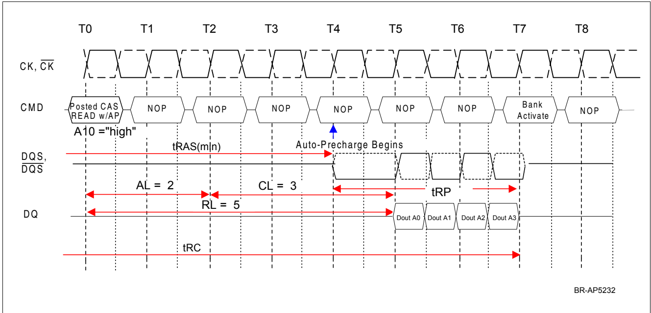
Figure 42 Read with Auto-Precharge Example 2, followed by an Activation to the Same Bank ( t_{RAS} Limit): RL = 5 (AL = 2, CL = 3), BL = 4, t_{RTP} \leq 2 clocks
