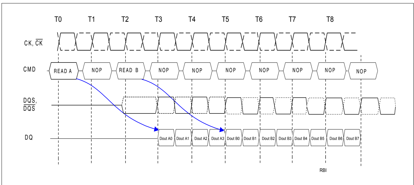
Figure 33 Read Interrupt Timing Example 1: (CL = 3, AL = 0, RL = 3, BL = 8)
