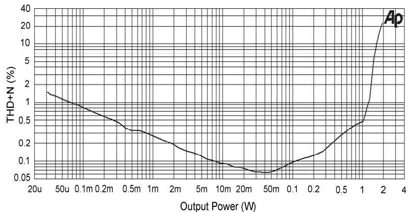
THD+N v.s. Output Power (1kHz input with 8\Omega load)
