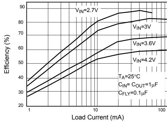
Fig. 8 Efficiency vs. Load Current
