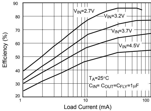
Fig. 7 Efficiency vs. Load Current
