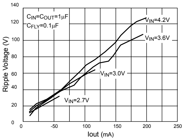
Fig. 9 Ripple Voltage
