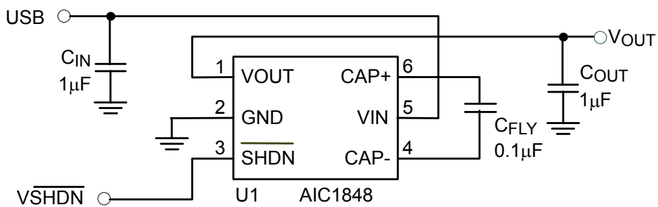
Fig. 17 Regulated 5V from USB
