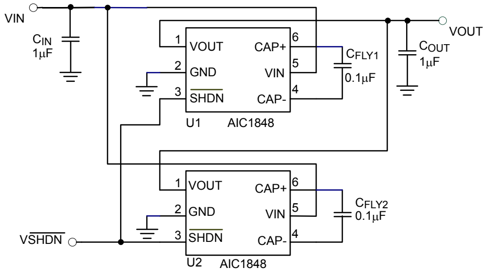
Fig. 16 Parallel Two AIC1848 to Obtain the Regulated 5V Output with large output current.
