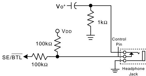
Figure 2: SE/BTL input selection by phonejack plug
