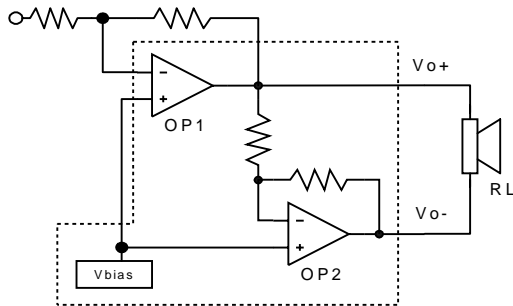
Figure 1: APA0710/1 power amplifier internal configuration
